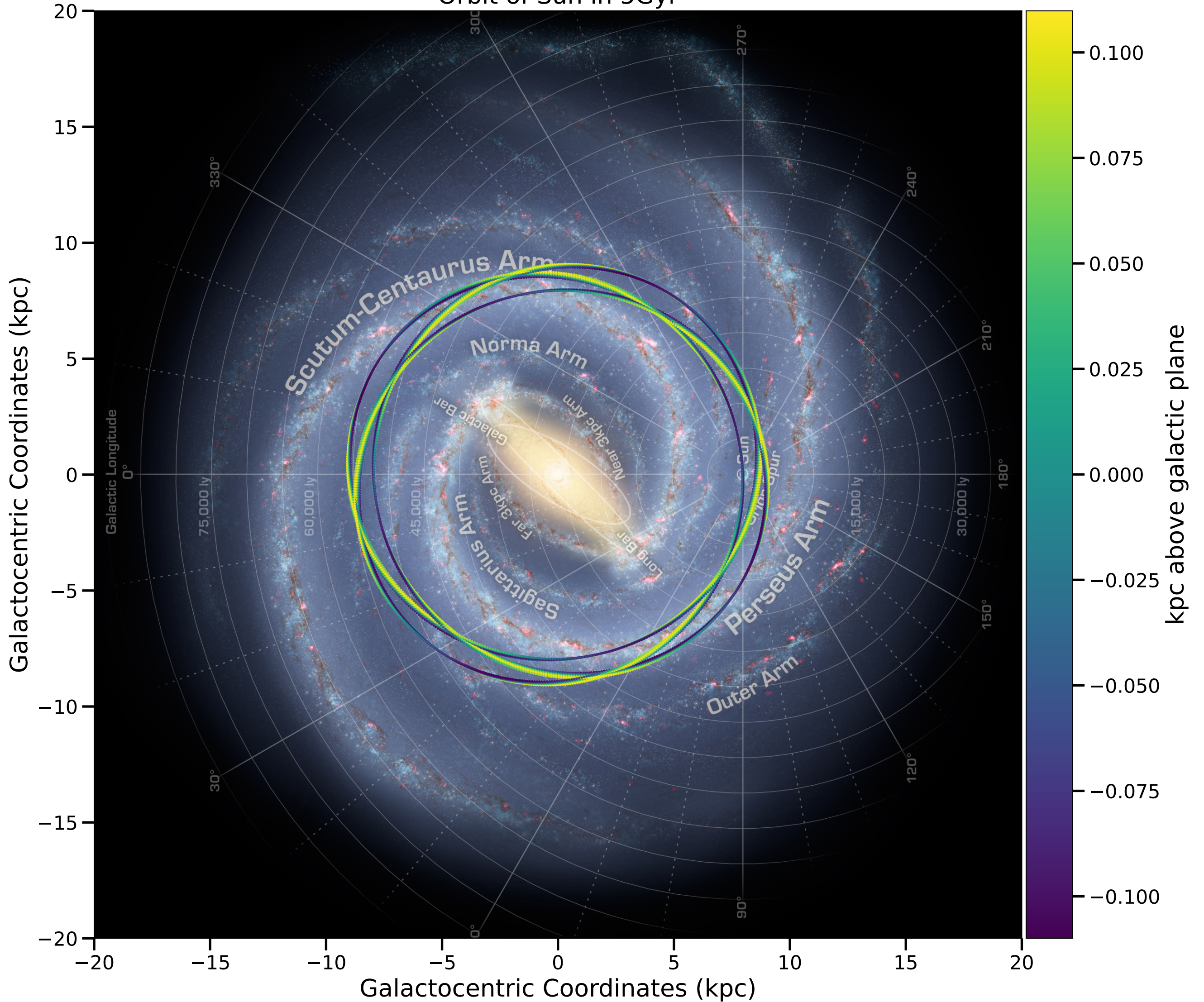
Orbit of Sun in 5Gyr
