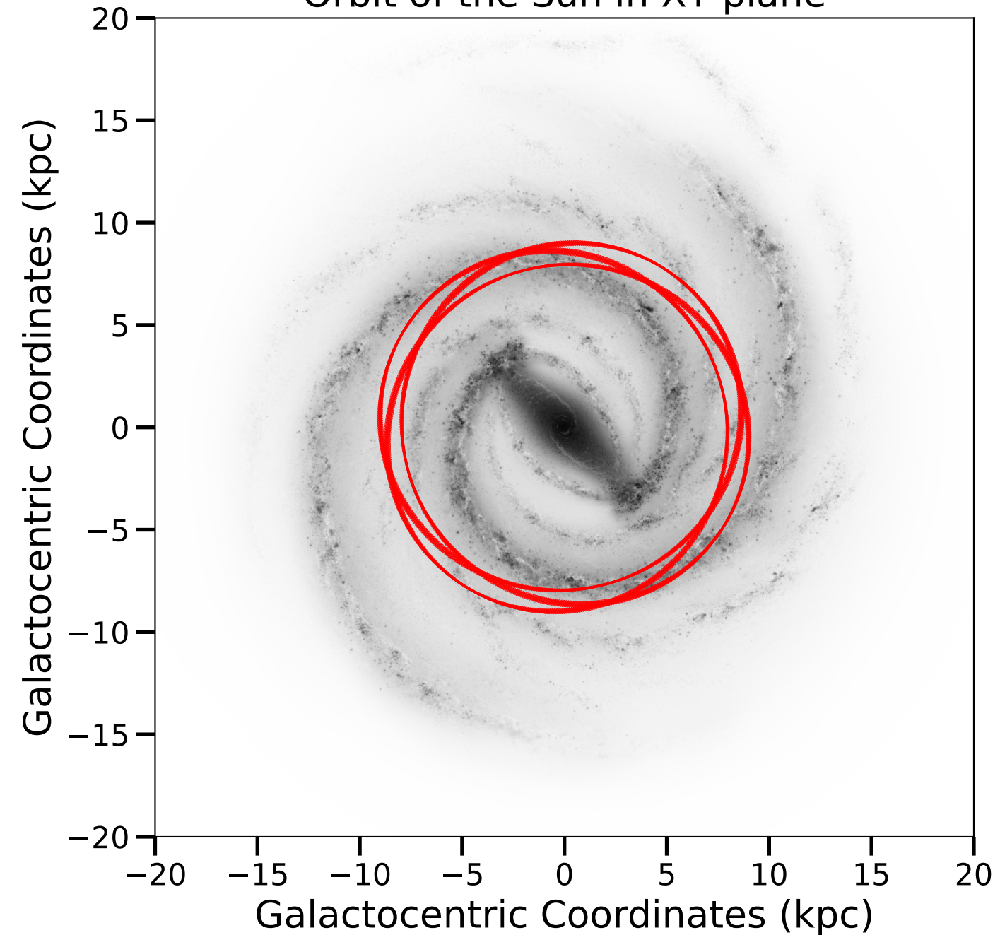
Orbit of the Sun in XY plane
