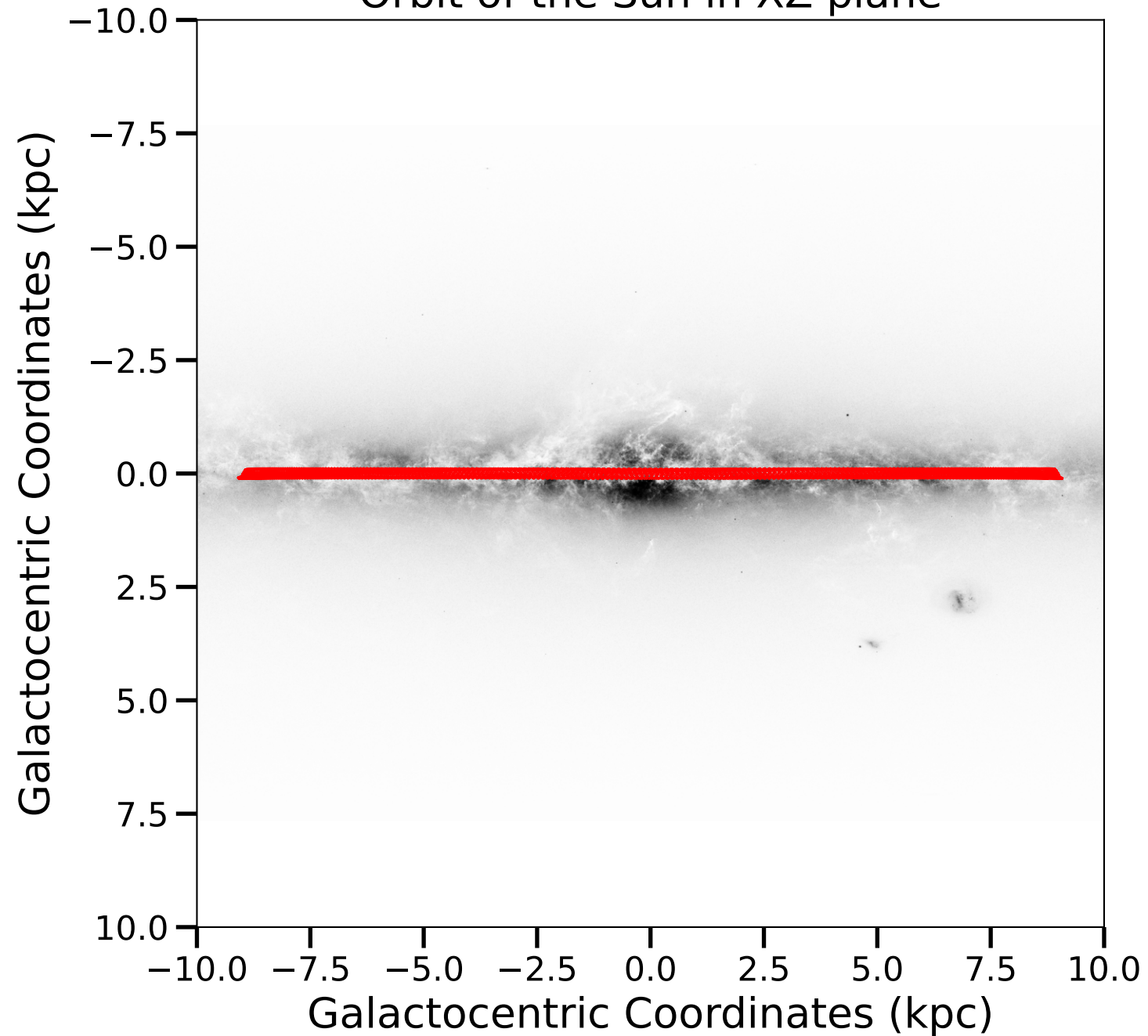
Orbit of the Sun in XZ plane
