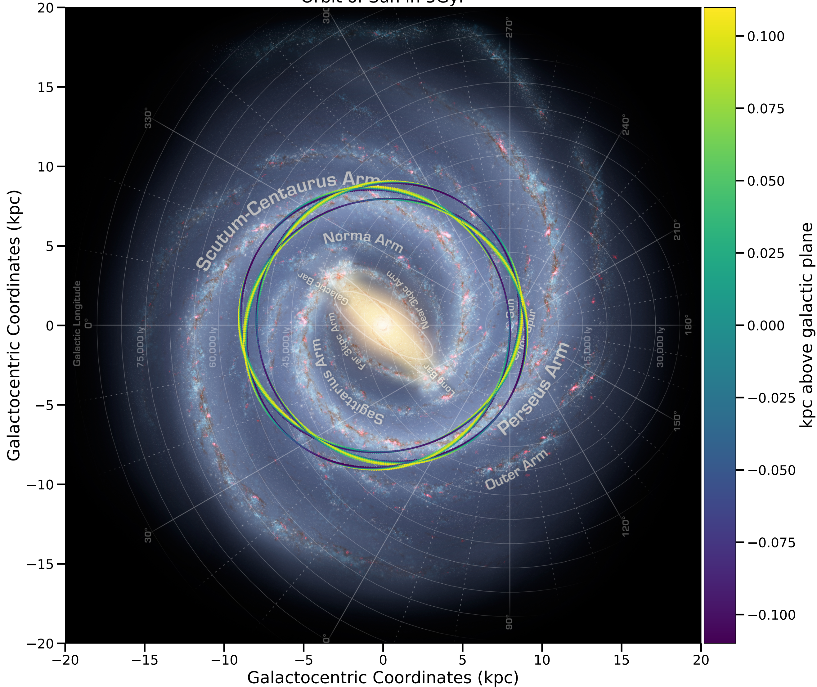
Orbit of Sun in 5Gyr
