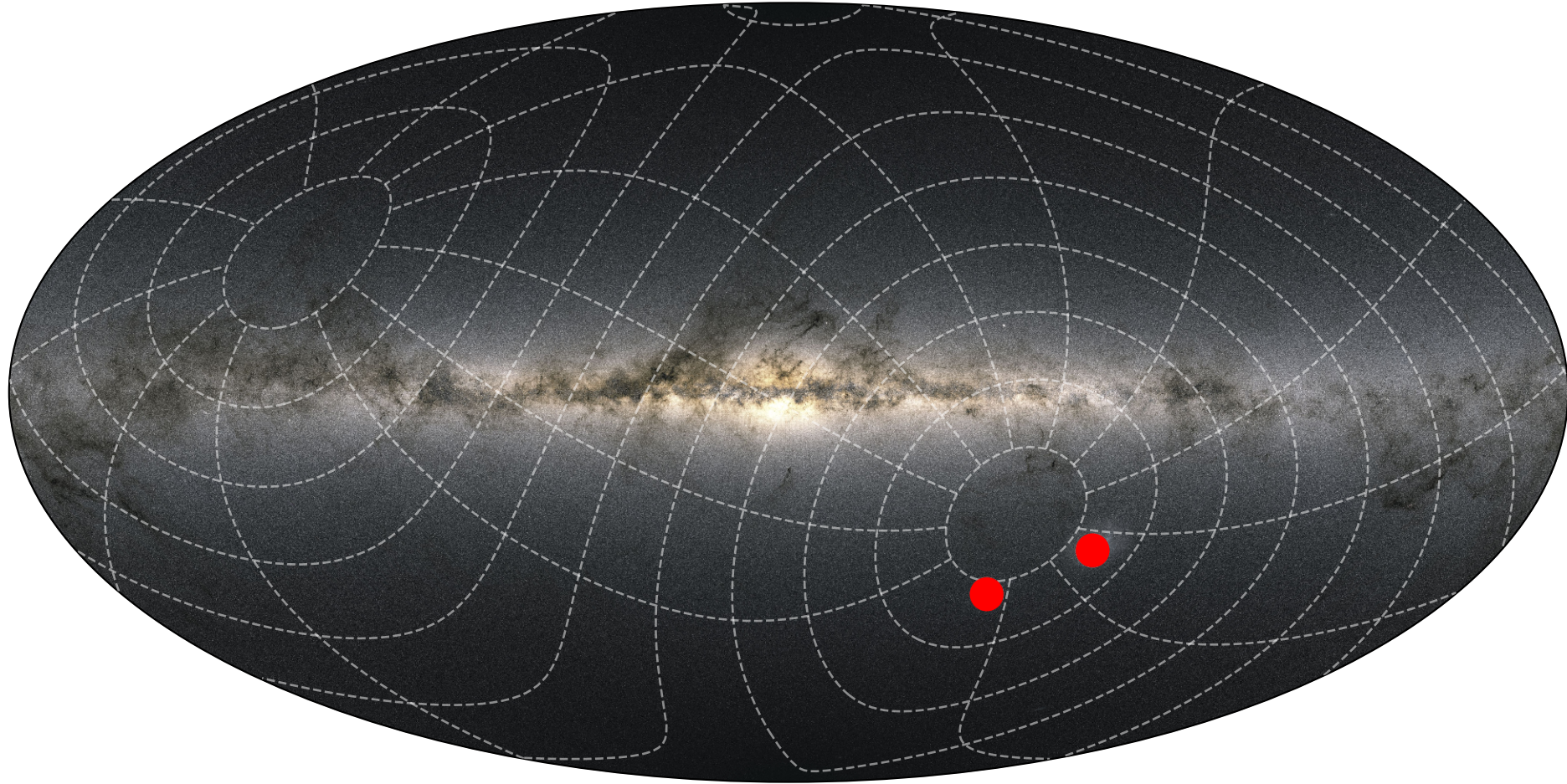
LMC and SMC in red dots with RA/DEC Grid
