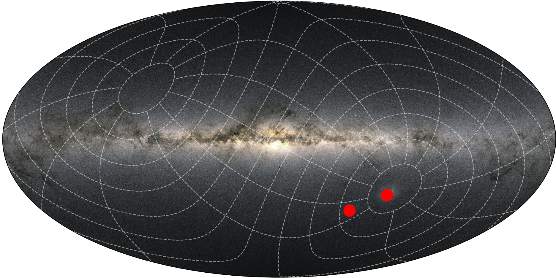
LMC and SMC in red dots with Ecliptic Grid
